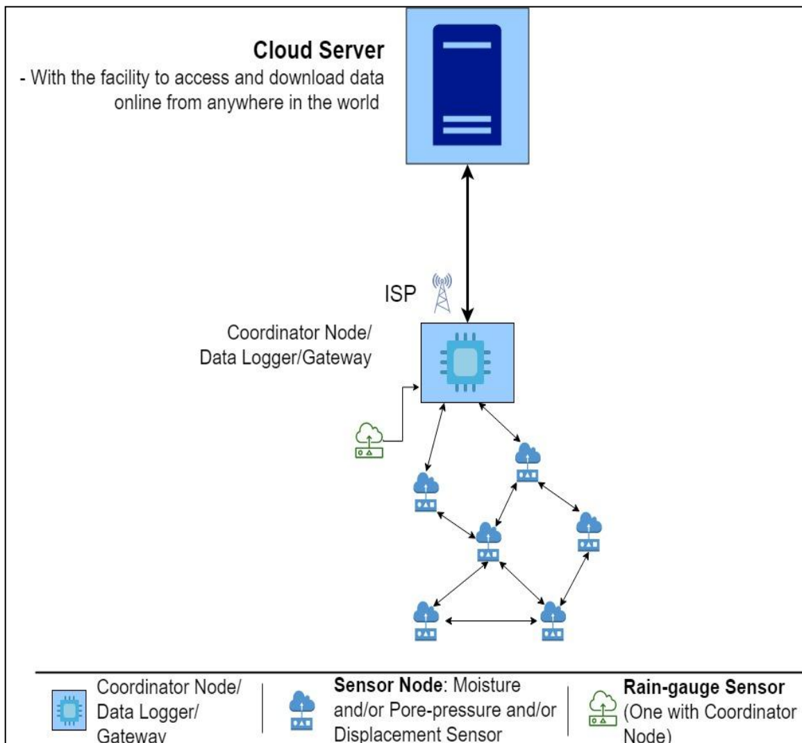
Fig.2. Network Architecture with Mesh Topology (Multi-hop) between Coordinator Node and Sensor Nodes
