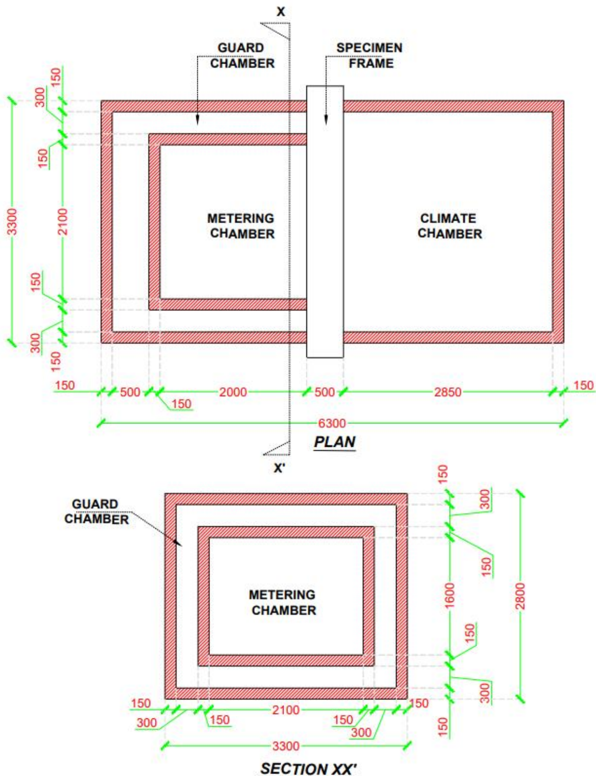
Figure 3: Guarded Hot Box type Apparatus dimensions (in mm)
