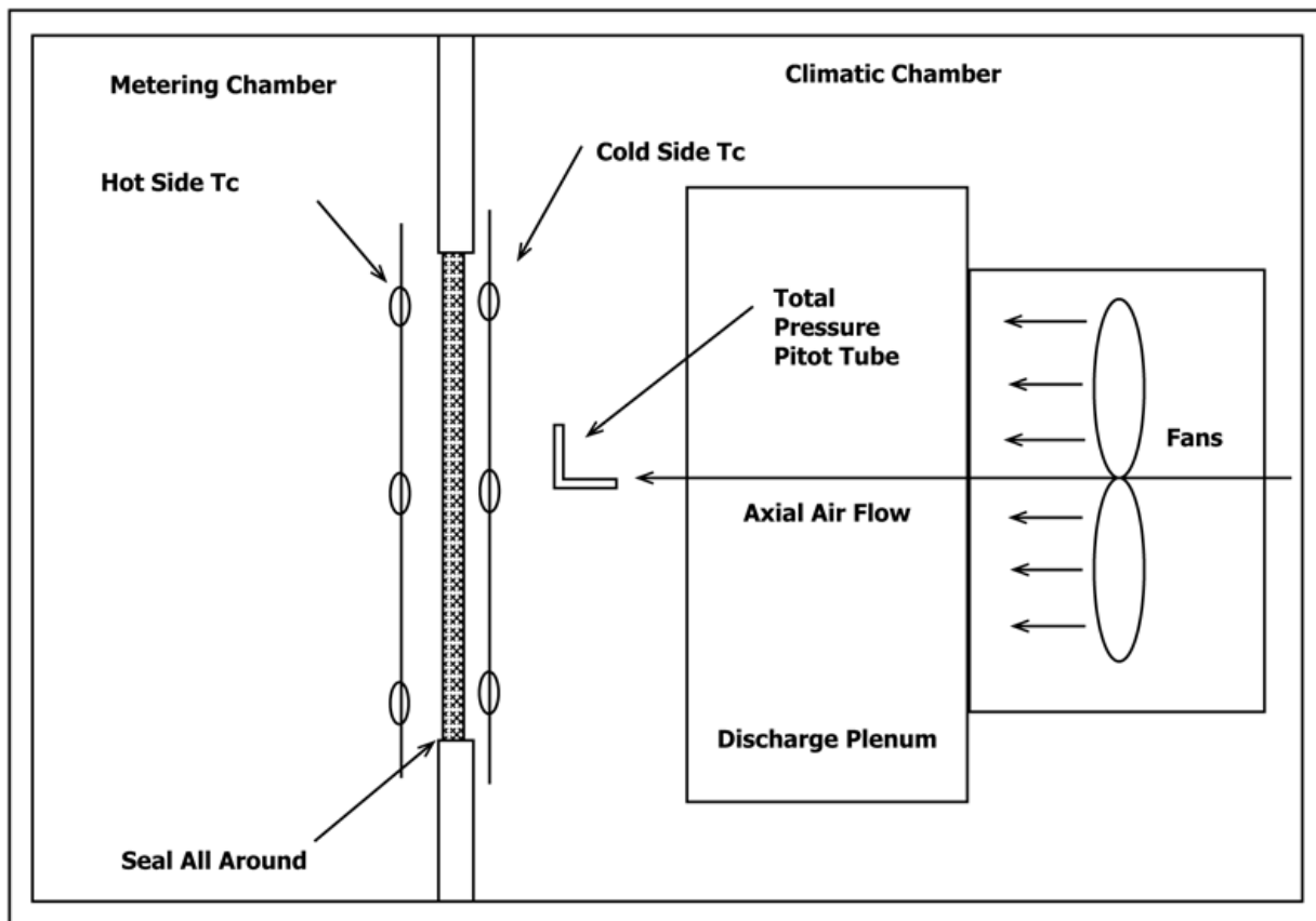
Figure 4: Hot Box Arrangement for perpendicular air flow
