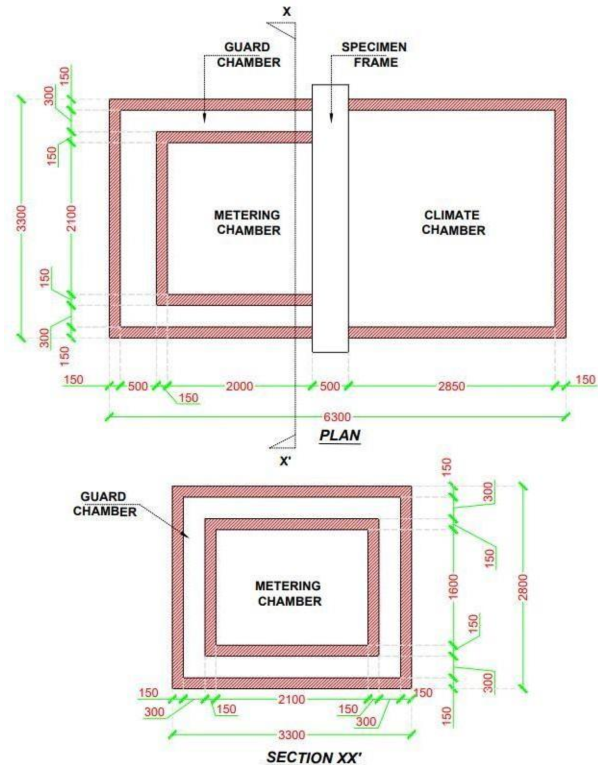
Figure 3: Guarded Hot Box type Apparatus dimensions (in mm) Specifications of Metering Chamber:
