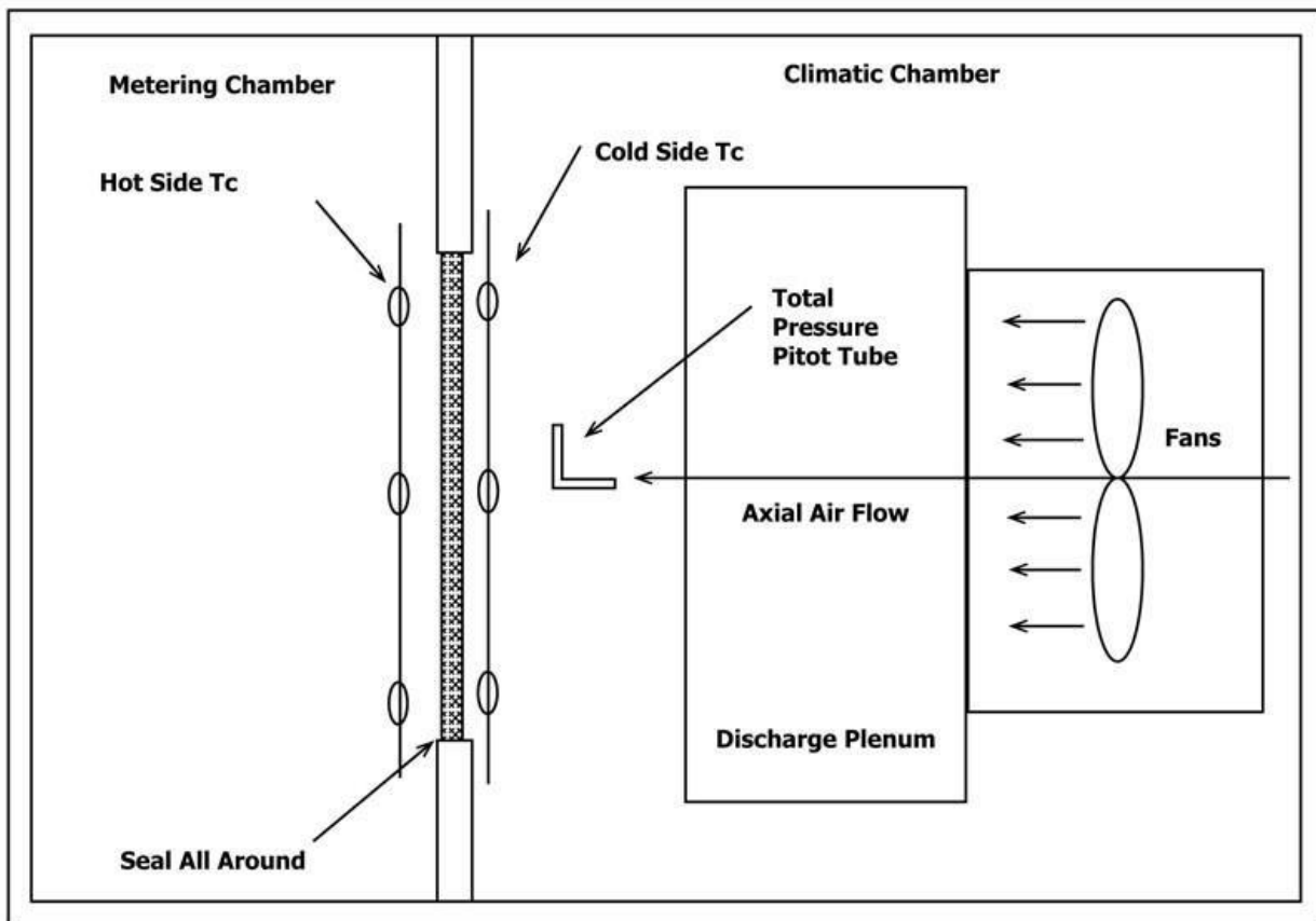
Figure 4: Hot Box Arrangement for perpendicular air flow Air Handling Unit (AHU)
