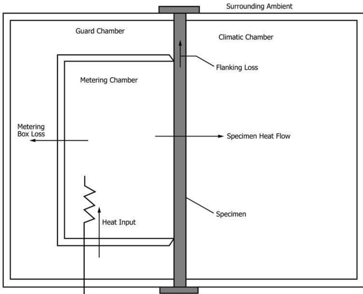
Figure 2: Typical Guarded Hot Box Apparatus
